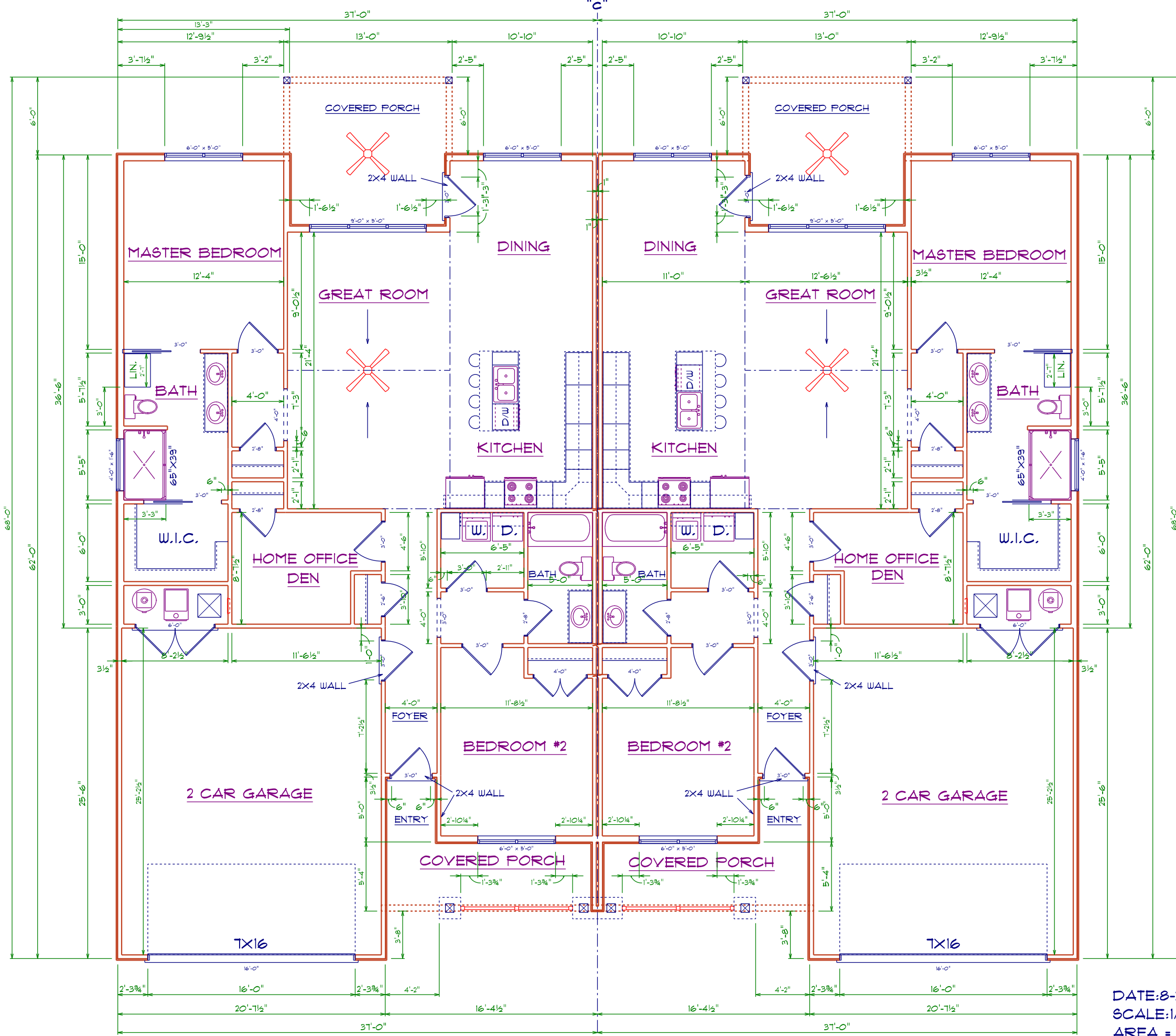
FLOOR PLAN
